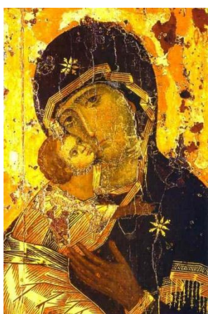
Fig. 2. The Mother of God. The situation denoted by the number ДВА=ДО+УА
